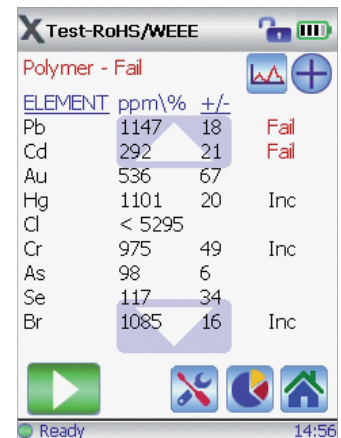
Pass/Fail and composition screen
