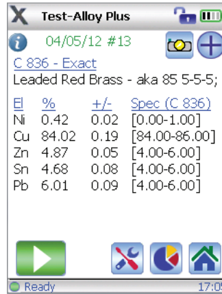
Grade Match Messaging in real time
